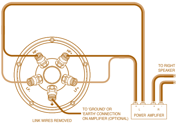
FIG. 3 BI-WIRE MODE AND EARTH (GROUND) LEAD CONNECTION
