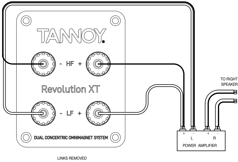
Fig.3 Bi-Wire Mode
