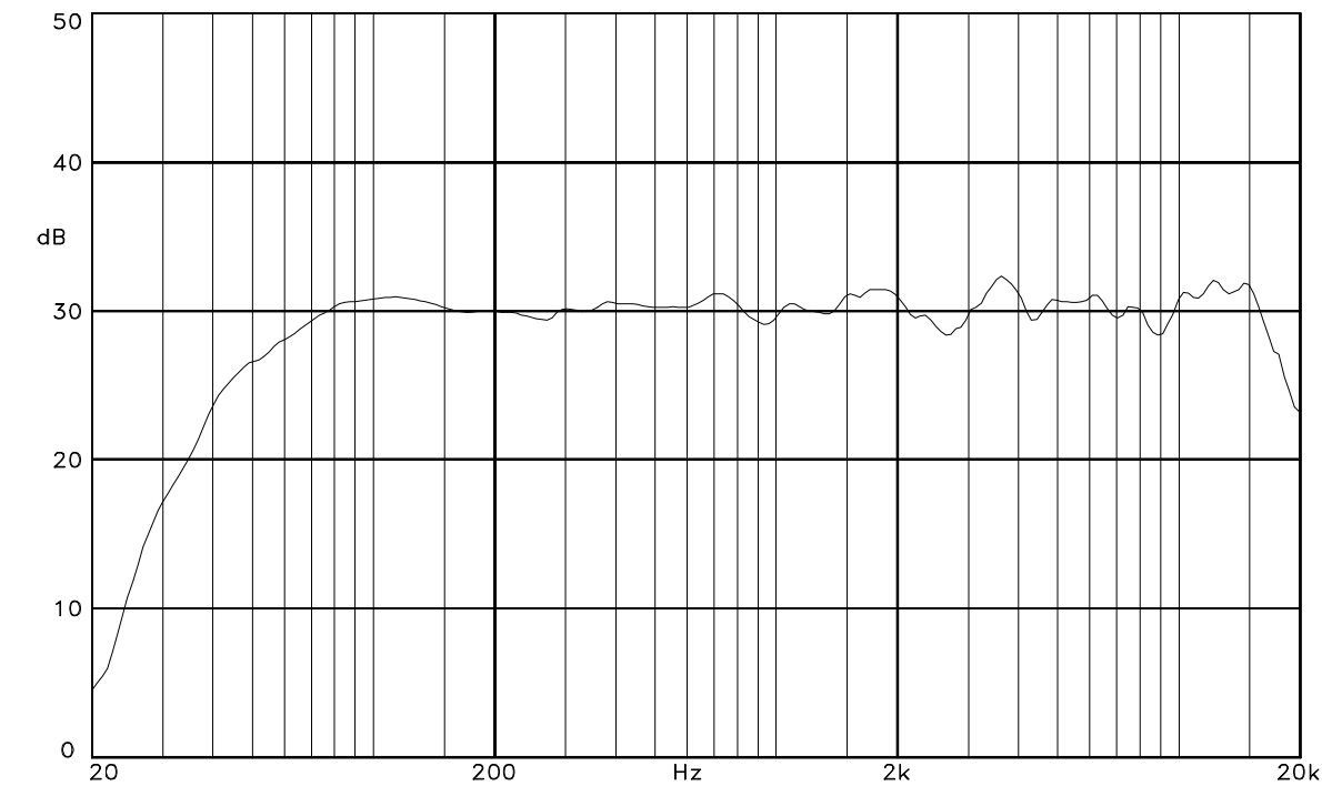
Figure 1. On axis anechoic response.
