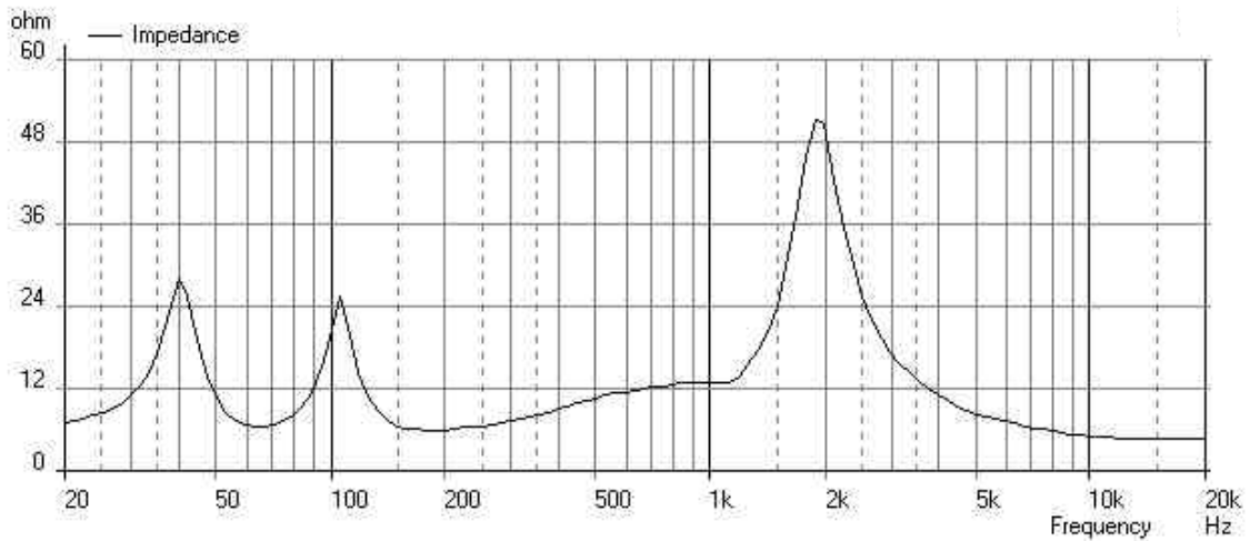
Impedance
