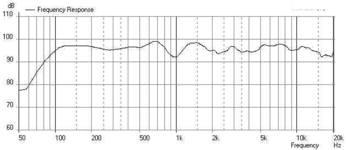
Unprocessed Anechoic Frequency Response, 1 watt @ 1 metre
