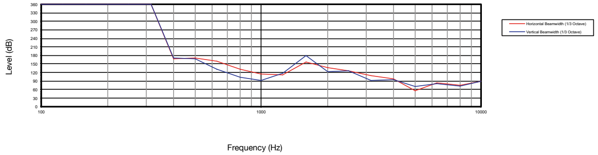
Beamwidth vs Frequency
