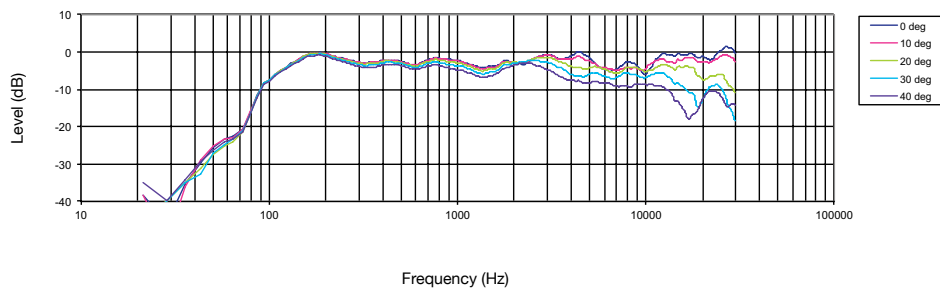
Horizontal off-axis Frequency Response
